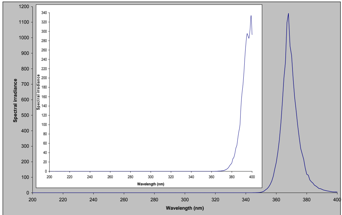
Figure 1. Mean spectral irradiance of Torch A at 100 cm ( \text{mW m}^{-2} \text{nm}^{-1} ), insert showing Torch B
